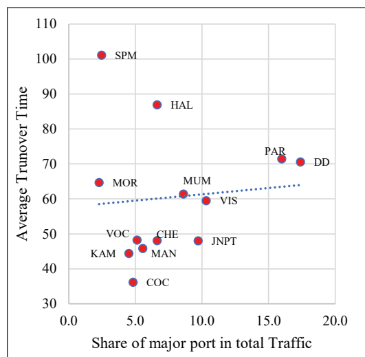
Figure 33: Relationship between the Traffic volume and Turnover Time
